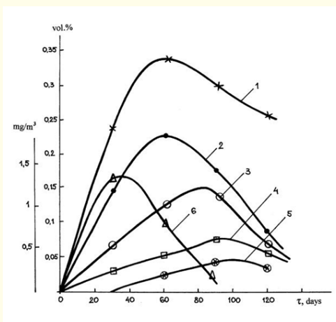
Figure 3: Experimental dynamics of toxic and greenhouse gas emissions from a “laboratory MSW micro-dump”. 1 - carbon dioxide (vol. %); 2 - methane (vol. %); 3 - ammonia (mg/m3); 4 - hydrogen sulfide (mg/m3); 5 - hydrogen chloride (mg/m3); 6 - formaldehyde (mg/m3).
