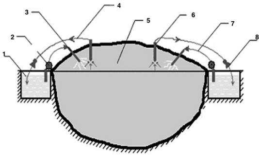
Figure 6: Technological scheme for extinguishing an unequipped MSW landfill with lime suspension \text{Ca}(\text{OH})_2 : 1 - Mixing tank (cistern) for the preparation and storage of lime slurry [\text{Ca}(\text{OH})_2] ; 2 - Powerful pump, supplying (under pressure) lime suspension from the tank to the injector (up to 60 \text{ m}^3/\text{h} ); 3 - Injector (pipe section 4-6 m long and 0.1 m in diameter with perforation and a pointed end) for injecting the suspension directly into the smoldering center in the body of the landfill; 4 - Pipeline for the removal of combustible and toxic gases from the body of the landfill (they are pumped into the tank with \text{Ca}(\text{OH})_2 for neutralization); 5 - MSW landfill body; 6 - Powerful vacuum pump (gas capacity up to 1 \text{ m}^3/\text{s} ); 6 - Perforated suction metal pipe (like injector, pos. 3) for venting gases from the landfill body; 7 - pipeline for supplying the suspension to the injector; 8 - Powerful vacuum pump (gas capacity up to 1 \text{ m}^3/\text{s} ) for suction of hot and toxic gases from the body of the landfill near the smoldering center (they are pumped into a tank with \text{Ca}(\text{OH})_2 for neutralization).
