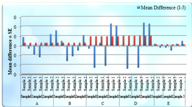
Figure 2: Post Hoc pair wise comparison between different samples at various dimensions (Tukey's HSD Test).
